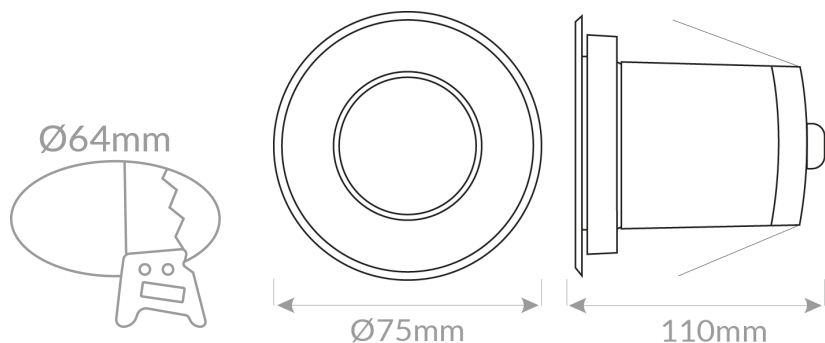
REF: 89153 3 Salidas
